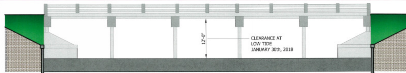
EXISTING BRIDGE ELEVATION
