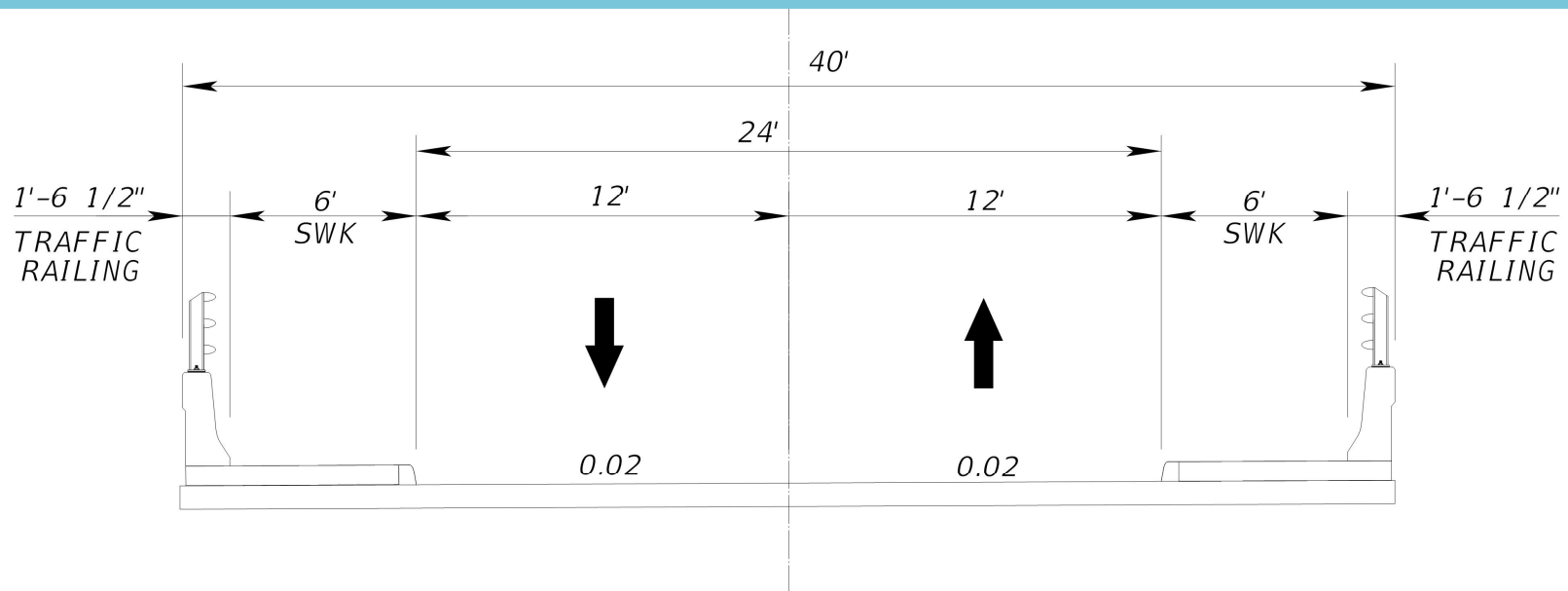
SE 5TH AVE BRIDGE
