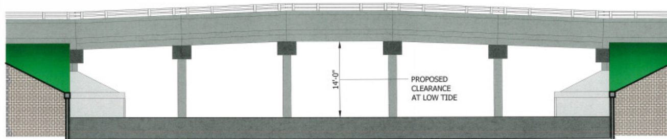
PROPOSED BRIDGE ELEVATION
